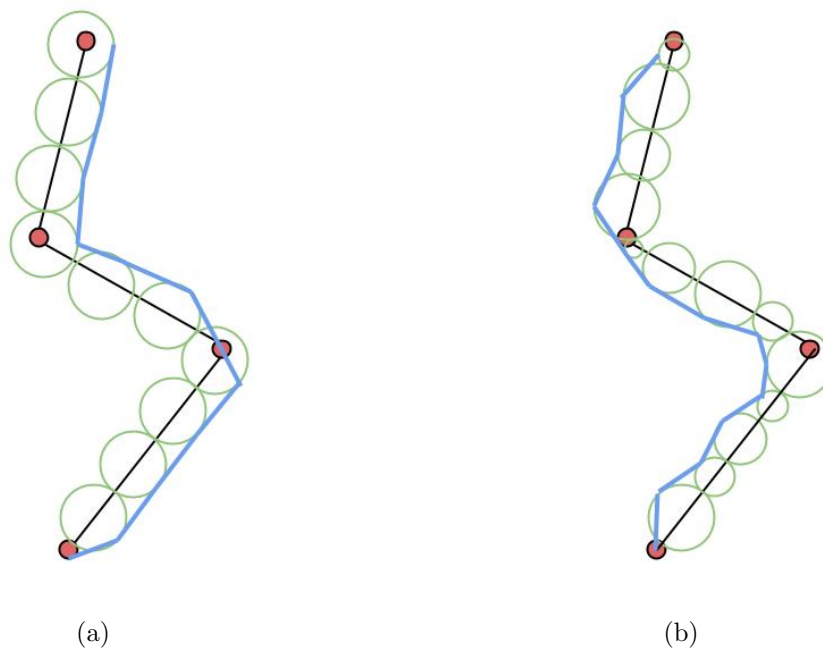
Figure 4.11: Showing circle diversification. (a) image shows a path (blue) generated from circles of equal size. (b) image shows a path generated with circles of variable size.
